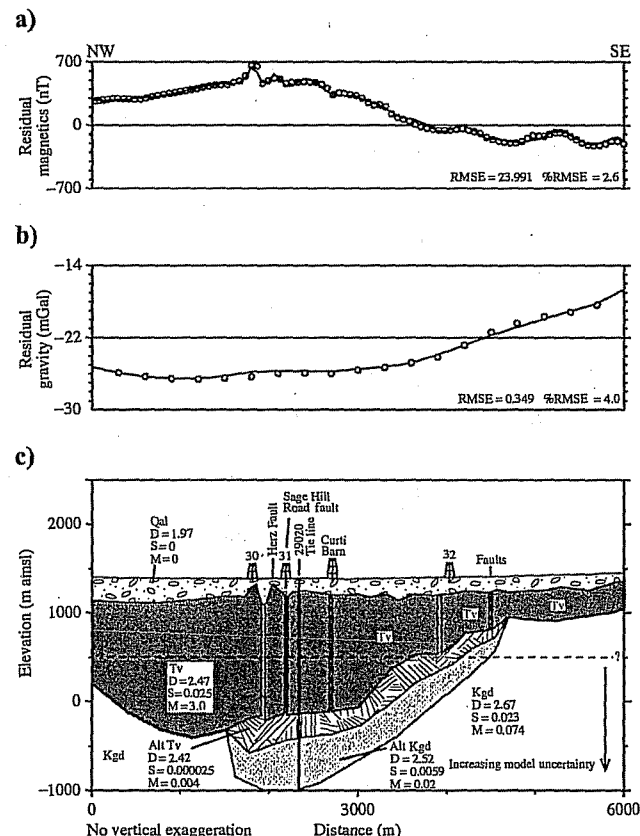
Figure 6. Profile 20330 cross section as computed by 2.75D forward modeling of gravity and aeromagnetic data. (a) Observed (dots) and fitted (solid line) residual reduced-to-pole aeromagnetic anomalies. (b) Observed (dots) and fitted (solid line) residual Bouguer anomalies. (c) Geologic cross-section with model block properties. Key as in Figure 5.
